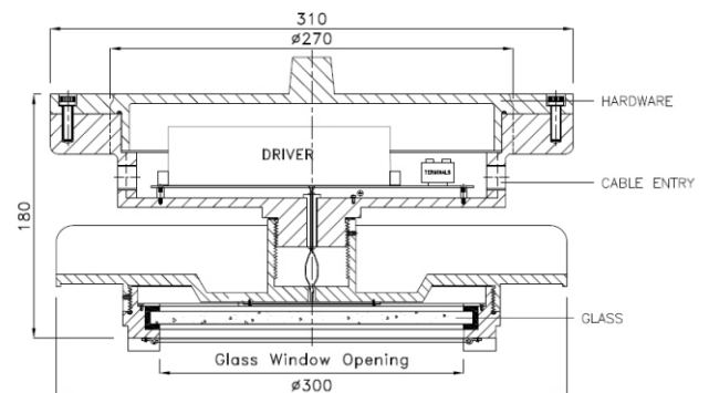
SECTIONAL VIEW OF FLOOD LIGHT FITTING SECTION -- B-B
