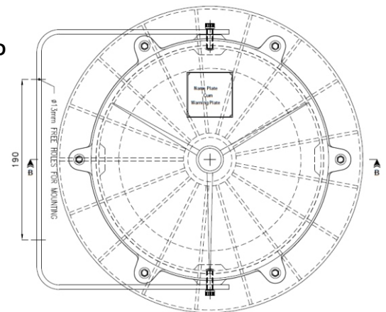
Plan View of Flood Light Fitting (TYPE - 2)
